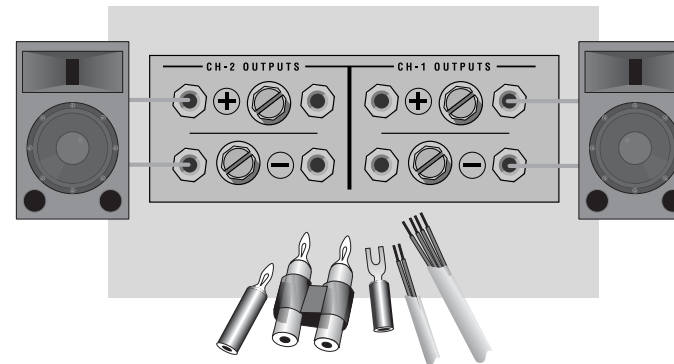
Figure 3.5 Output Connector Wiring
